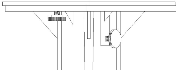
Figure 3 - Tripod bracket
